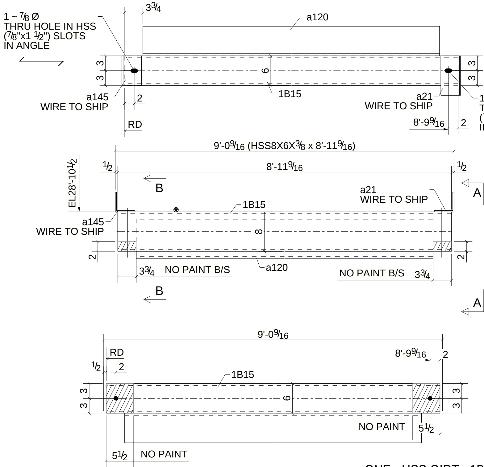
ONE - HSS GIRT - 1B15
